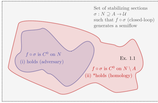
FIG. 1. A summary of the context and contribution of this work. (1a) When the control system (see § 1.1) is such that \mathcal{U} \rightarrow X is a vector bundle, with X oriented, then, the homology condition (ii) is stronger than the adversary condition (i). (1b) When \mathcal{U} \rightarrow X is a fiber bundle (e.g., a sphere bundle), there are examples showcasing that this ordering fails (see Example 1.1). Nevertheless, the system studied in Example 1.1 does admit a stabilizing controller, however, one that is merely continuous on N \setminus A (not on all of N ). (2) Indeed, we show that the homology condition (ii) holds true for stabilizing control systems with mild discontinuities on A , hence one could argue that (1b) displays shortcomings of the adversary condition, not of the homology condition. (1c) To overcome these shortcomings, we develop the spherical adversary condition (iii); this adversarial condition accommodates mild discontinuities, handles Example 1.1 and is again implied by the homology condition.
